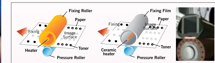
Conventional Roller Fixing Method On-Demand Fixing Method
